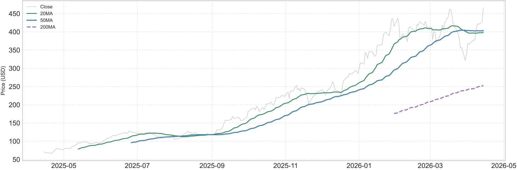
MU — Closing Price with Moving Averages (1 Year)
